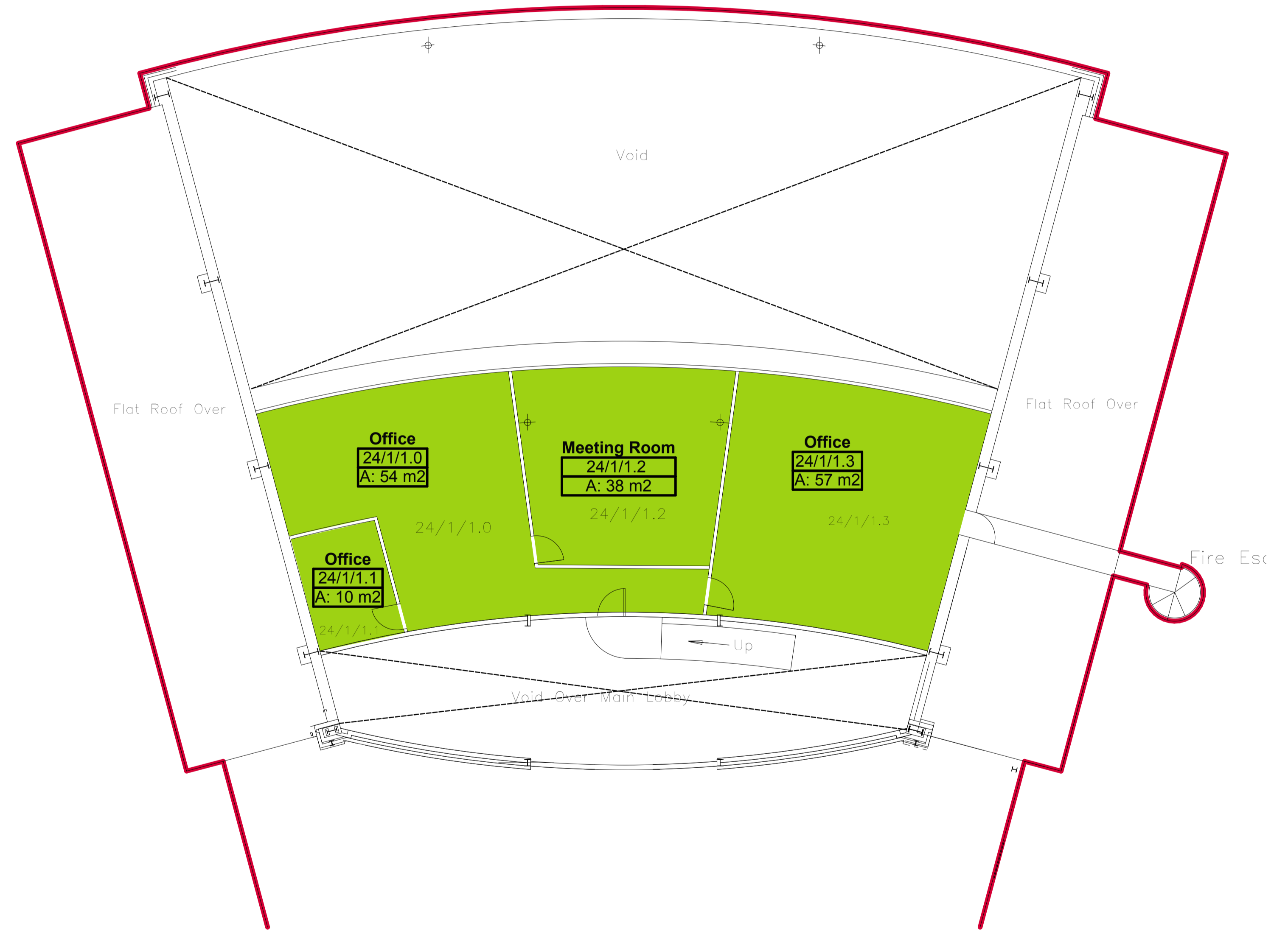
First Floor- Area take off 1:100
